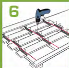
6 Prepare the remaining decking boards.
