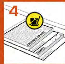
4 Lay the drainage and the upper sub-base.
