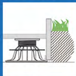
Buttress finish
