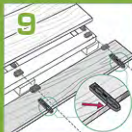
9 Attach the final components.
