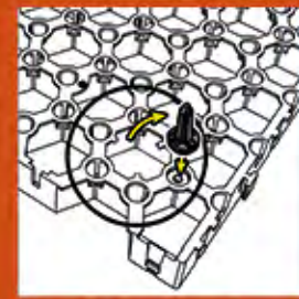
When laying on a slope, please cut and use the anchoring pins, and insert them into the underside of the tile for extra grip.
